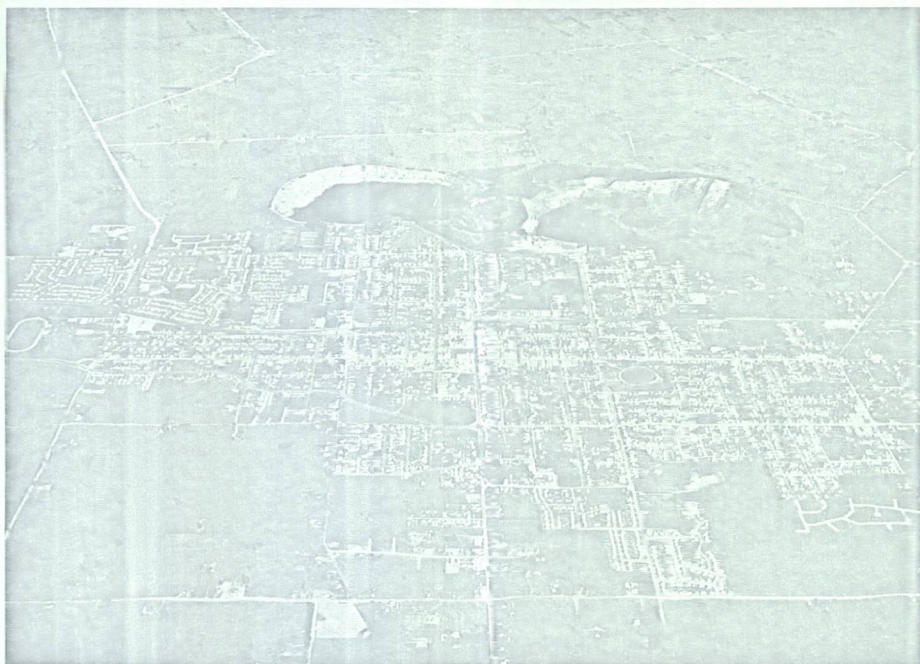
FIG. 10 - Mount Gambier. Around Blue Lake on the left bedrock can be seen between the water and the overlying pyroclastics. (Photo kindly supplied by the Town Clerk, Mount Gambier).
