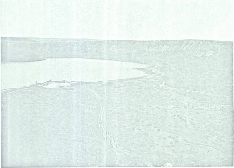
FIG. 6 - Zuni Salt Lake. General view of the floor and rampart. (Photo C. D. Ollier).
