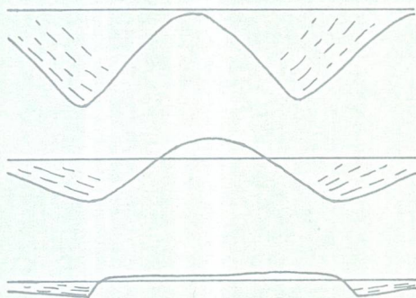
FIG. 15 - Diagram to show the continuous series from maar to Noorat type volcanoes.
