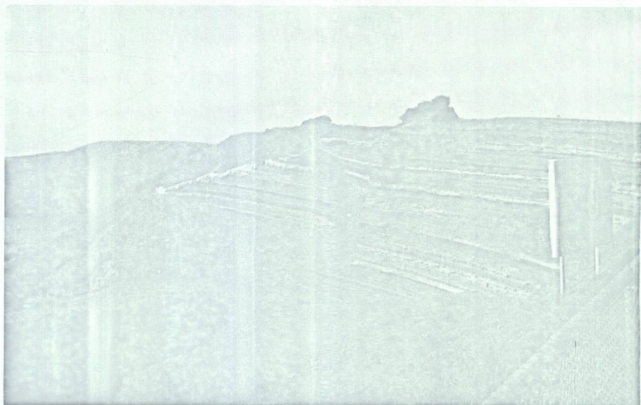
FIG. 5 - Bedded tuff, Tower Hill. (Photo C. D. Ollier).
