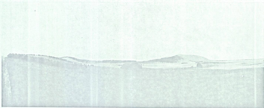
FIG. 17 - Mount Warrnambool. (Photo C. D. Ollier).
