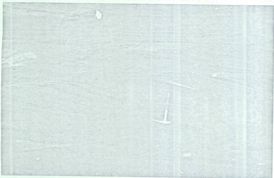
FIG. 12 - Cross-bedded tuff, Purumbete. (Photo C. D. Ollier).
